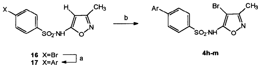
Scheme 4. Synthesis of N -(4-bromo-3-methyl-5-isoxazolyl)biphenylsulfonamides. (a) \text{ArB(OH)}_2 , EtOH, \text{C}_6\text{H}_6 , 2M \text{Na}_2\text{CO}_3 , \text{Pd(Ph}_3\text{P)}_4 (cat.), 80^\circ\text{C} ; (b) NBS, \text{CH}_2\text{Cl}_2 , 0^\circ\text{C} .
