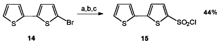
Scheme 3. (a) t -BuLi, \text{Et}_2\text{O} /pentane, -78^\circ\text{C} , 20 min; (b) \text{SO}_2 , -78^\circ\text{C} ; (c) NCS/THF, -78^\circ\text{C} to room temp.
