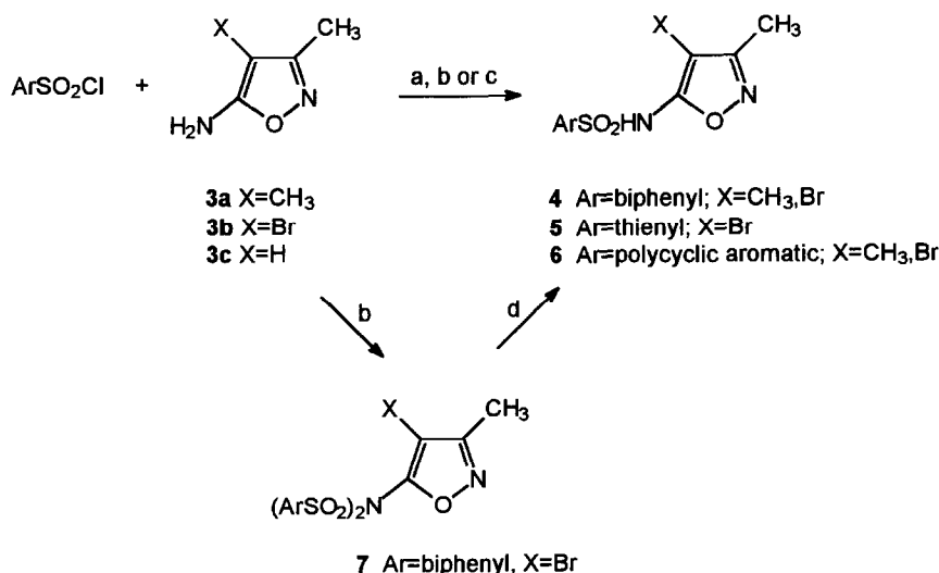
Scheme 1. General synthesis of N -isoxazolyisulfonamides. (a) Pyridine; (b) pyridine, N,N -dimethylaminopyridine (cat.); (c) NaH. THF, 0–25°C; (d) NaOH, THF/H 2 O, 45°C.
