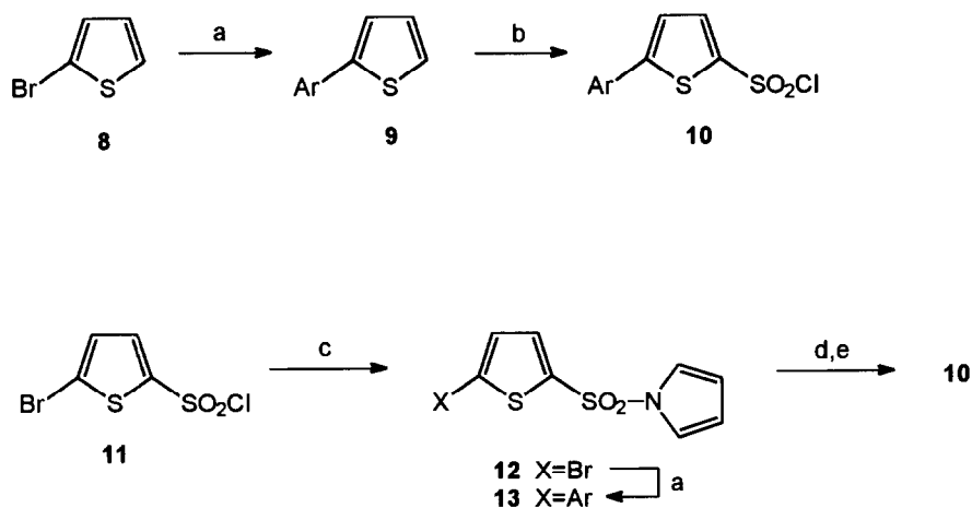
Scheme 2. Synthesis of 5-Aryl-2-thiophenesulfonyl chlorides. (a) \text{ArB(OH)}_2 , EtOH, \text{C}_6\text{H}_6 , 2M \text{Na}_2\text{CO}_3 , \text{Pd(Ph}_3\text{P)}_4 (cat.), 80^\circ\text{C} ; (b) \text{ClSO}_3\text{H} , \text{PCl}_5 , \text{POCl}_3 ; (c) pyrrole, NaH, THF, 25^\circ\text{C} ; (d) NaOH, MeOH, reflux; (e) \text{PCl}_5 , \text{POCl}_3 , 25^\circ\text{C} .
